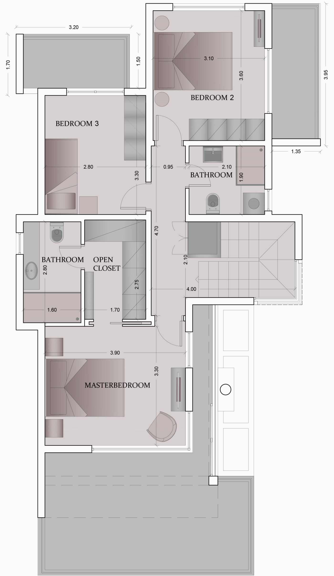
FIRST FLOOR AREA 65.80 sq.m.
