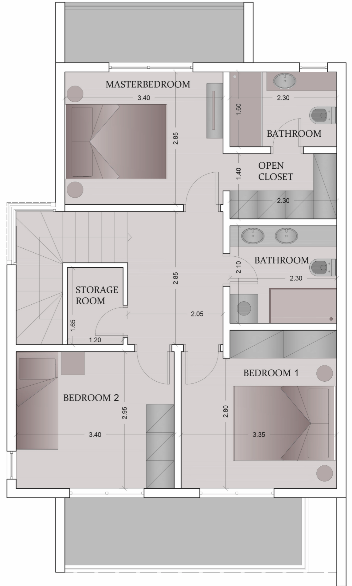
FIRST FLOOR AREA 63.40 sq.m.
