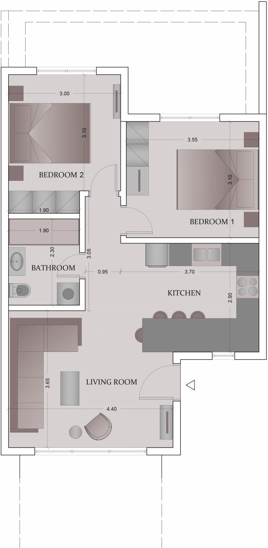
GROUND FLAT 3 AREA 65.80 sq.m.
